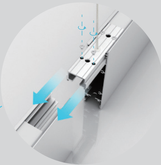
LH25 Connection (without end cap)
