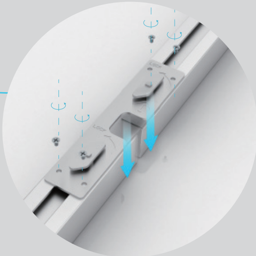
LS25 Connection (with end cap)
